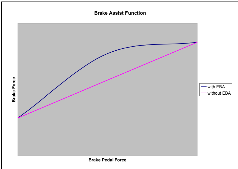
Figure 1: The EBA function
