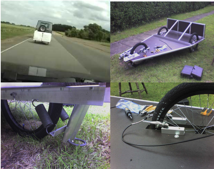
Figure 3: The trailer through driver's view in the track (top left), during development (top right) and details of the auto-brake mechanism (bottom left/right)
